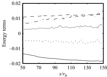
FIGURE 9. Axial variations over 50r_0 \leq x \leq 150r_0 of peak values across the jet of terms in the turbulent kinetic energy budget: - · - ·, mean flow convection; - - -, production; ·····, turbulence diffusion; — — —, pressure diffusion; —, dissipation (curves normalized by \rho_c u_c^3 \delta_{0.5} , \rho_c : centreline mean density).
