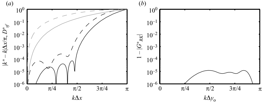
FIGURE 1. Representation using logarithmic scales: (a) phase error |k^* - k|\Delta x/\pi introduced by (—) the present 11-point finite differences and (---) the second-order central finite differences, and damping rate D_{sf}^* of (— — —) the present 11-point selective filter and (— — —) the second-order central filter for a wavenumber k on a uniform \Delta x grid; (b) damping rate 1 - |G_{RK}^*| due to time integration, per iteration, for a wavenumber k convected at the jet exit velocity u_j on the \Delta y_0 grid in the present LES.
