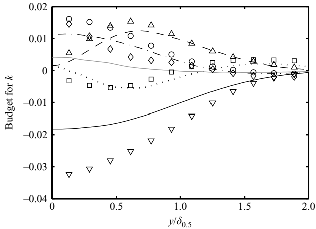
FIGURE 21. Budget for k across the self-similar jet, compared with data of Hussein et al. (1994): mean flow convection (---, LES; \circ , Hussein et al. ), production (---, LES; \triangle , Hussein et al. ), dissipation (—, LES; \nabla , Hussein et al. ), turbulence diffusion (·····, LES; \square , Hussein et al. ) and pressure diffusion (—, LES; \diamond , Hussein et al. ).
